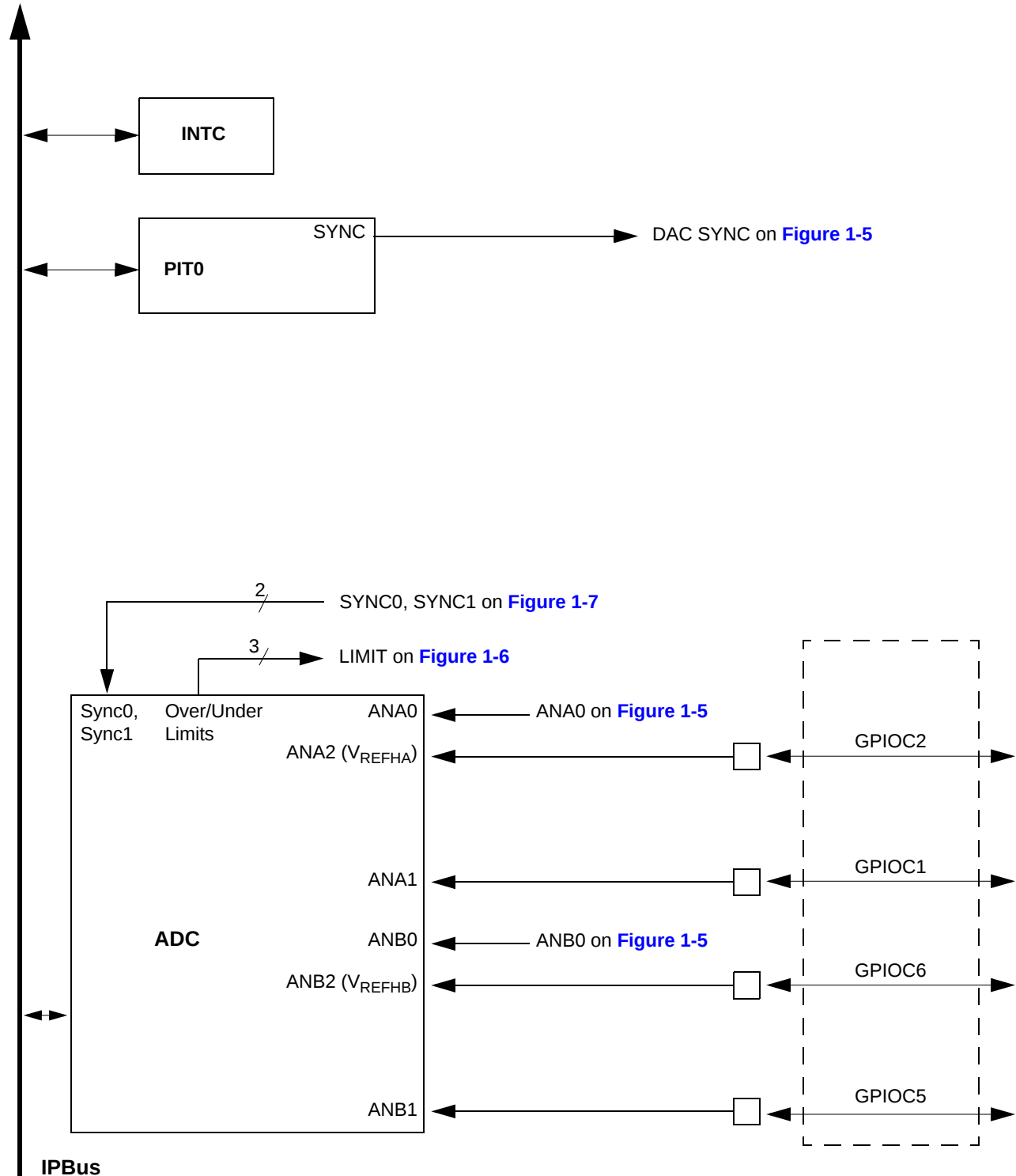
Figure 1-3 56F8023 I/O Pin-Out Muxing (Part 1/5)
